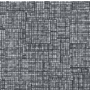
DAT131-154 DECODE
